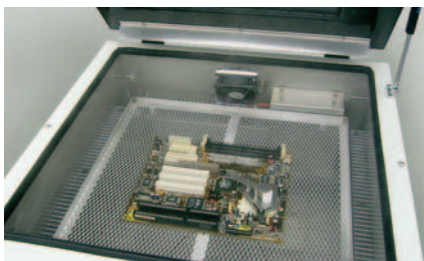
Work Piece Carrier with Assembly at Feed-In Position
