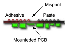
Misprints
